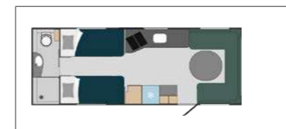
650 BSA Beds 2 x 195 x 88.5 cm Seating group 160/132 x 225 cm
