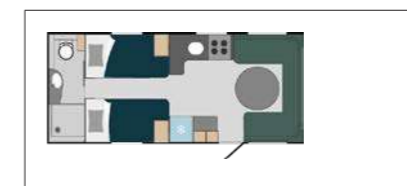
590 BS Beds 2 x 195 x 88.5 cm Seating group 160/132 x 225 cm
