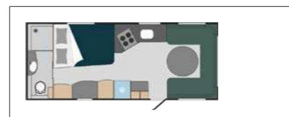
620 BFWA Bed 195 x 134/112 cm Seating group 160 x 225 cm
