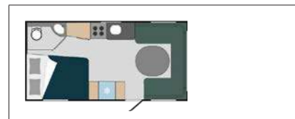
520 FD Bed 195 x 144/122 cm Seating group 160/132 x 225 cm
