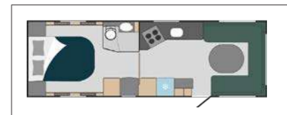
730 QA Bed 200x140 cm (electric) Seating group 188/160 x 225 cm
