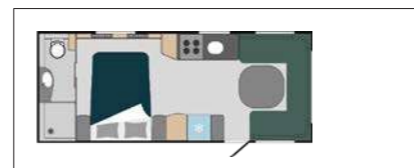
620 BQD Bed 195.5 x 140/125.5 cm Seating group 160/132 x 225 cm
