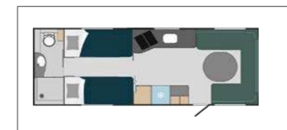
680 BSA Beds 2 x 195 x 88.5 cm Seating group 188/160 x 225 cm
