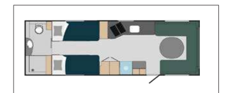
730 BSA Beds 2 x 195 x 88.5 cm Seating group 188/160 x 225 cm
