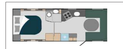
680 QA Bed 200x140 cm (electric) Seating group 160x225 cm
