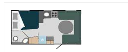
520 FW Bed 195 x 144/122 cm Seating group 160/132 x 225 cm
