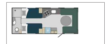
620 BSA NEW Beds 2 x 195 x 88.5 cm Seating group 160/132 x 225 cm
